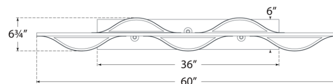
Bottom View
